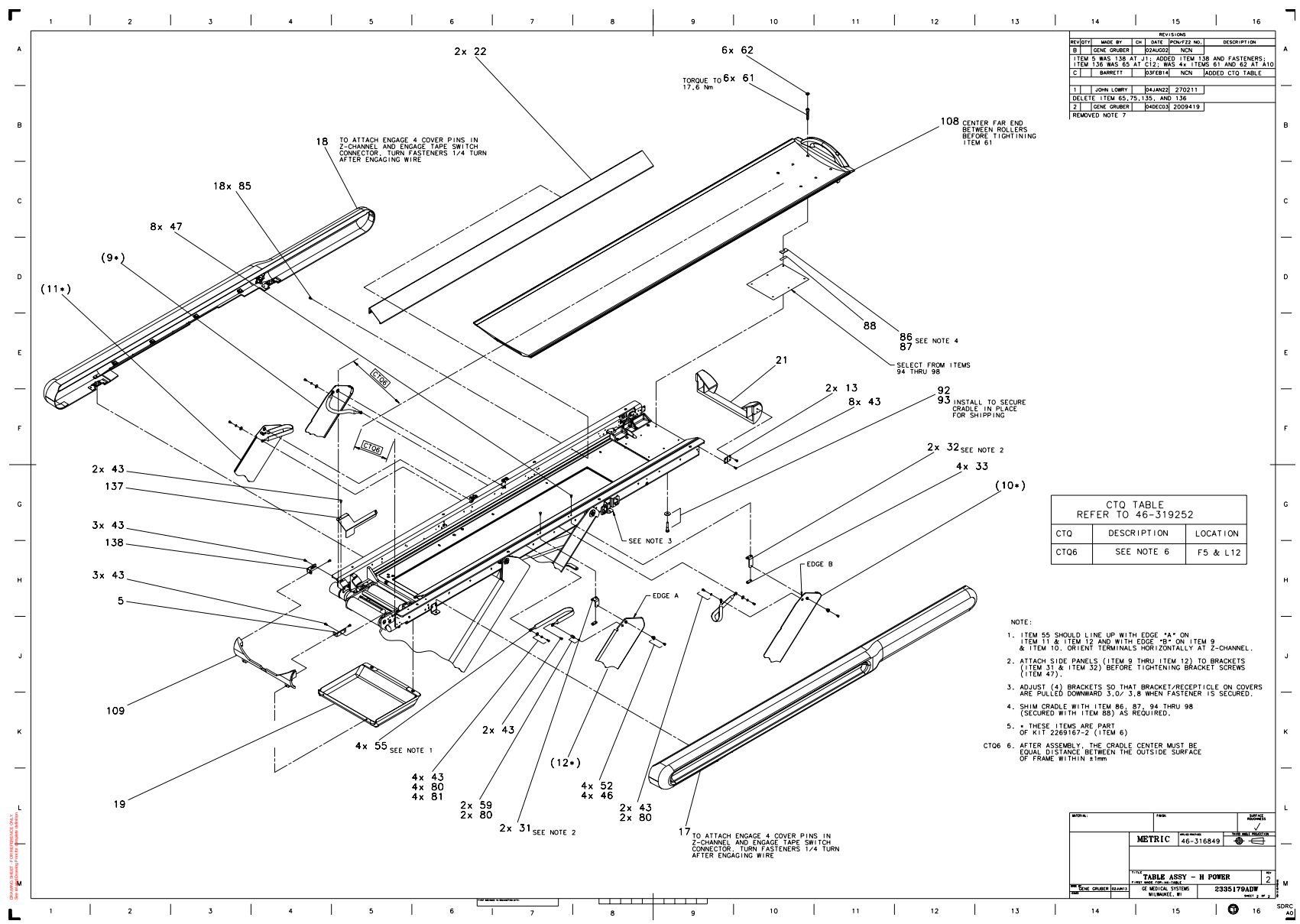
Figure 2-2 Table Assembly - H Power (2335179, sheet 2, rev 2)
