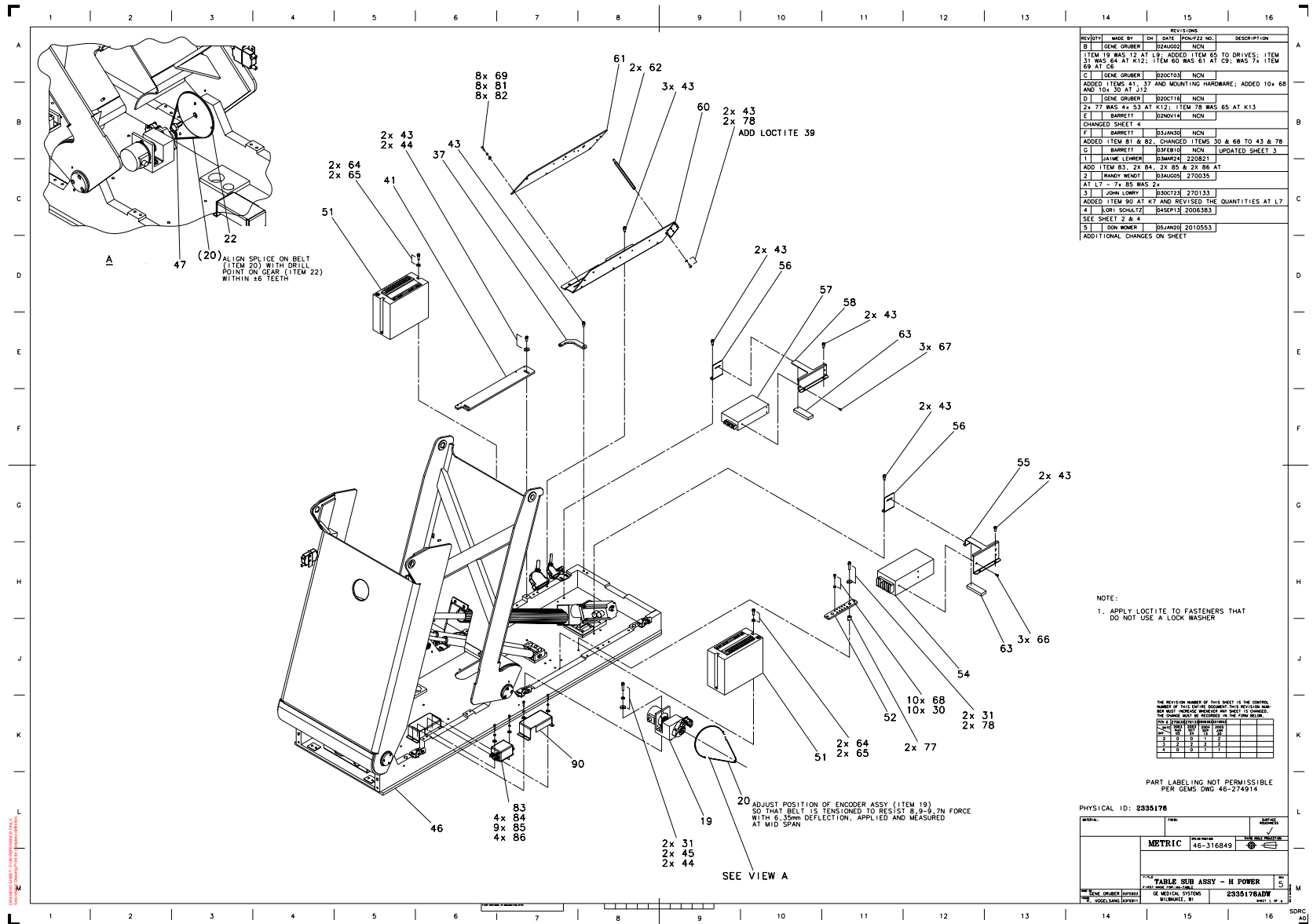
Figure 2-6 Table Subassembly (2335178, sheet 1, rev 5)
