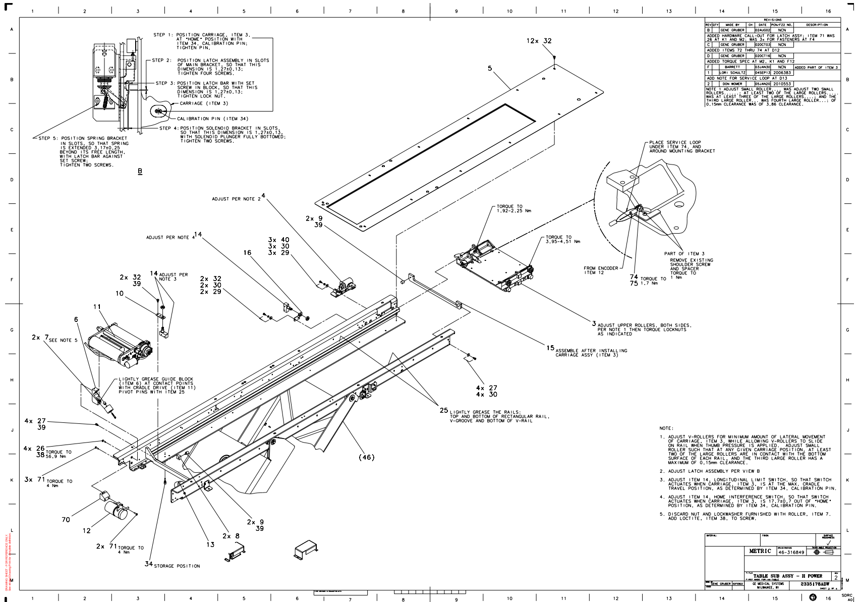
Figure 2-7 Table Subassembly (2335178, sheet 2, rev 2)
