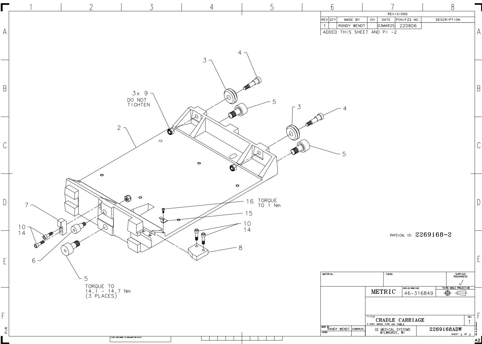
Figure 2-10 Carriage Assembly (2269168, sheet 2, rev 1)
