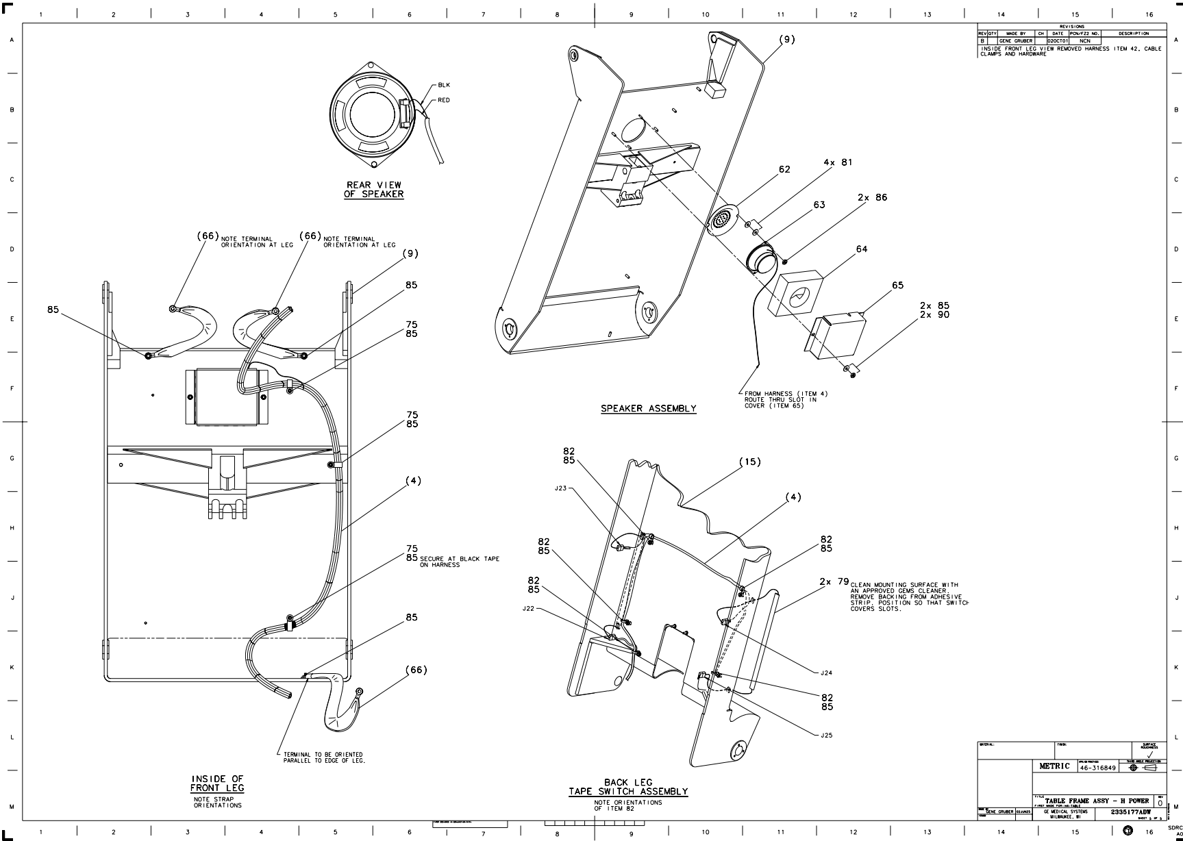
Figure 2-20 Table Frame Assembly (2335177, sheet 5, rev 0)
