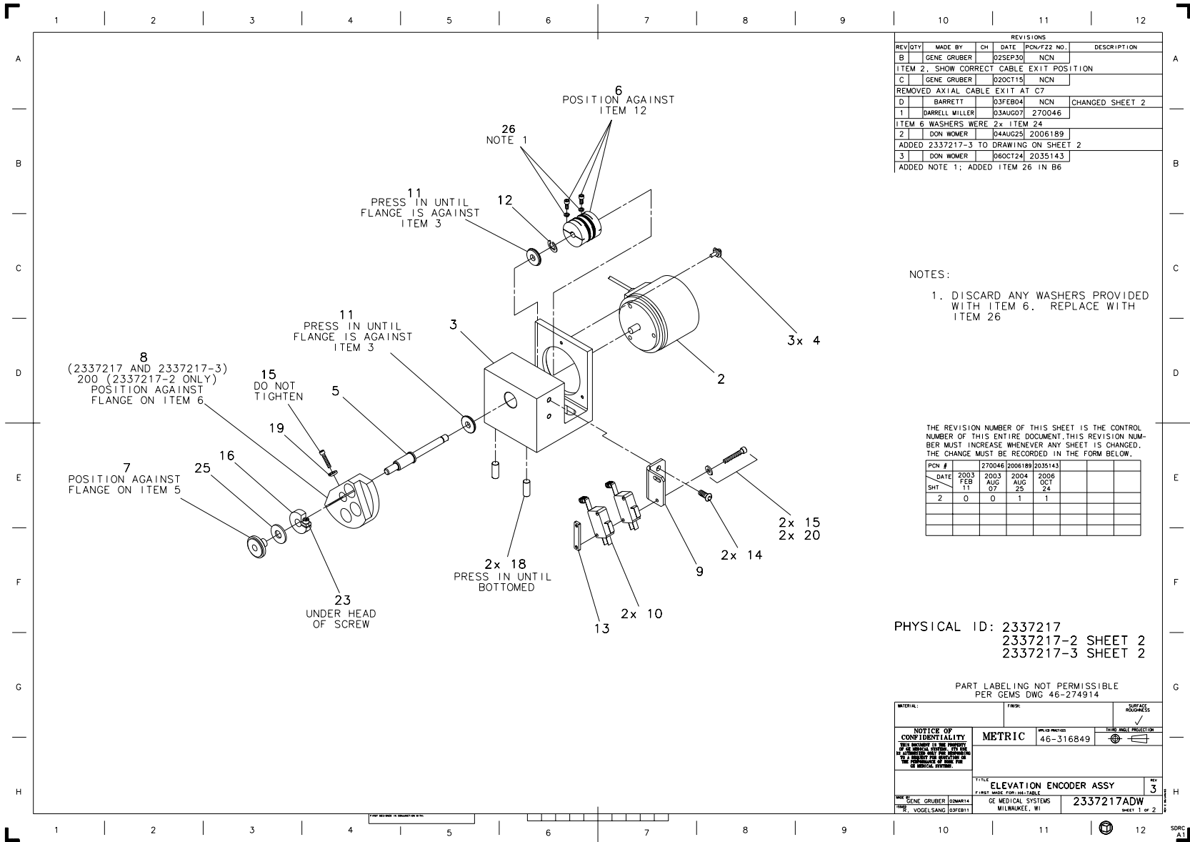
Figure 2-15 Encoder Assembly, Elevation - H Power (2337217, sheet 1, rev 3)
